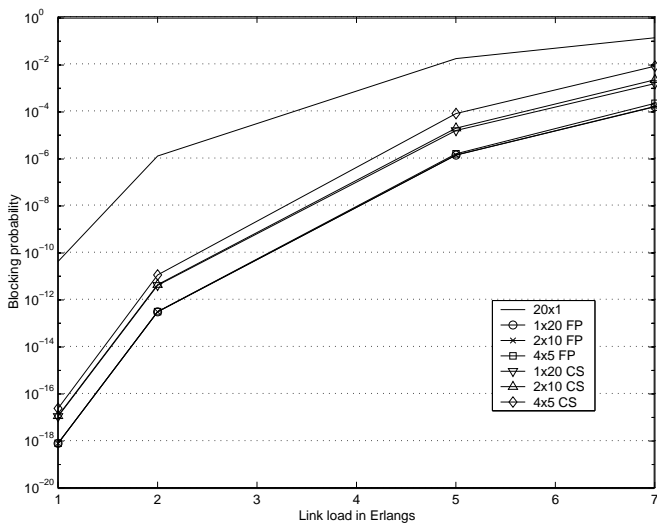
Fig. 11. Blocking probability versus link load for a 10-dimensional hypercube network.
