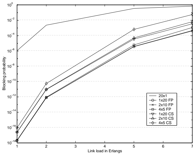
Fig. 10. Blocking probability versus link load for a 25x25 bi-directional mesh-torus network.
