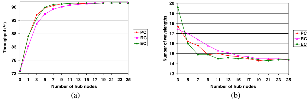
Fig. 4. (a) Network throughput as a function of the number of hub nodes for the 25 node network with W = 13 , \delta = 3 (b) Wavelength requirements for 100% throughput (throughput is less for RC heuristic) at \delta = 3 , as a function of the number of hub nodes for the 25 node network.
